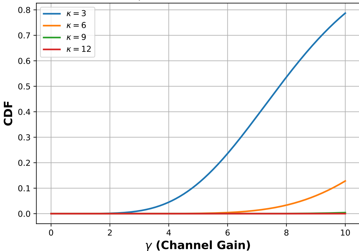
CDF of \gamma with d=2.0 , N_t=4 (MISO)
